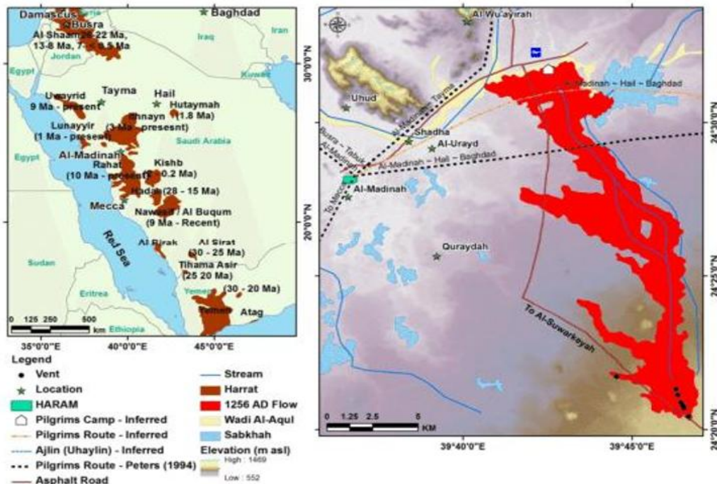
Figure (1) Regional map showing the distribution of the volcanic fields (harrats) across Arabia and the Levant (a). Map showing the location of the 1256 AD lava field relative to prominent geographic locations and historical pilgrimage routes.
